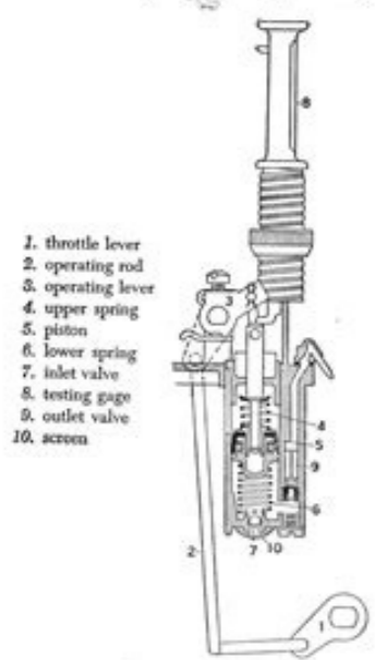
FIG. 12. Accelerator Pump
